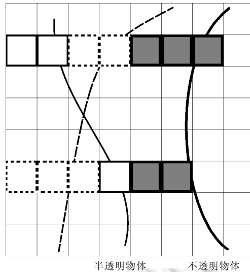
Fig.2 In ray casting steps of volume rendering, per-pixel depth sorting is applied to blend interlaced objects 图2 在体绘制的光线积分中采用了基于像素的深度排序,可以对交错的对象进行正确的混合绘制
