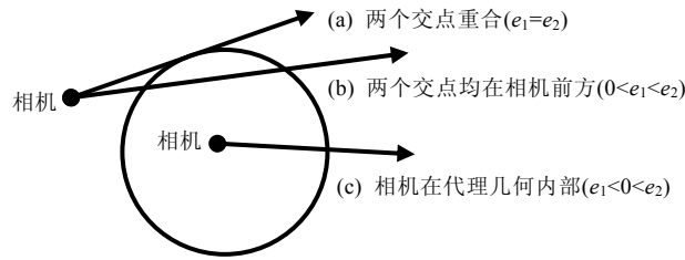
Fig.1 Three types of intersection points of casted ray and proxy geometry
