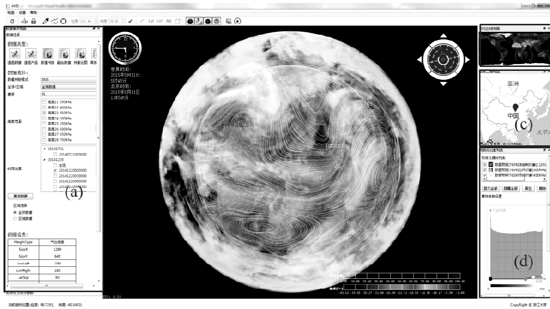
Fig.4 System interface. This scene contains streamlines of wind field, horizontal slice of temperature filed and volume rendering of relative humidity
