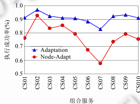
Fig.5 Successful execution ratio values of composite services
