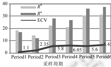
Fig.4 Distribution of ECV
