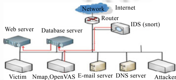
Fig.3 Topology of test network
