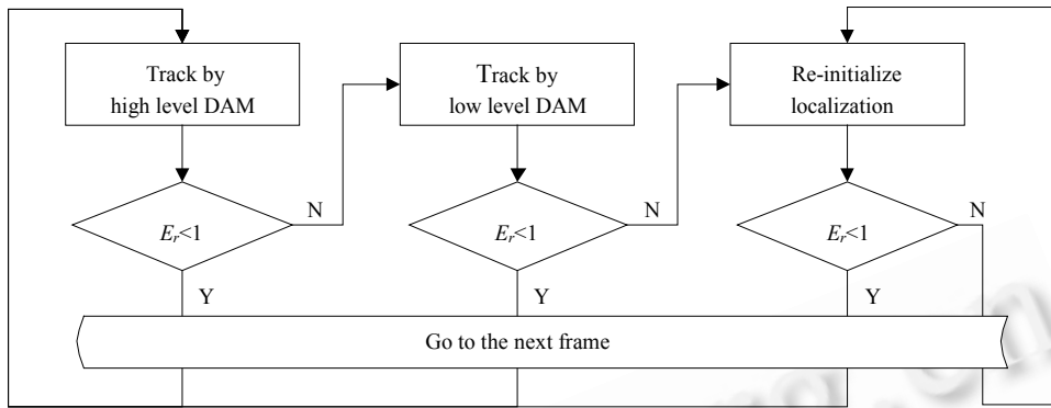
Fig.4 Flowchart of two-level DAM for facial feature point tracking 图 4 两层 DAM 人脸特征点跟踪框图
