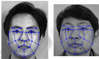
Fig.2 Using DAM to localize facial feature points
