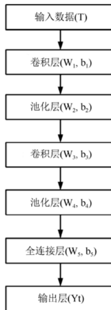
Fig.4 Structure of CNN model used in this paper
