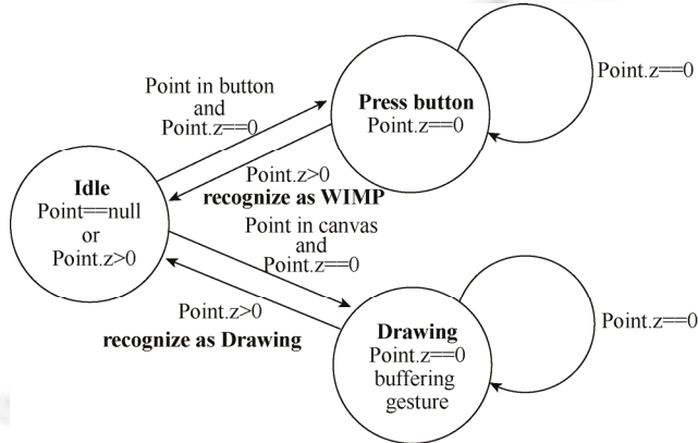
Fig.3 Identifying process of WIMP task and drawing task
