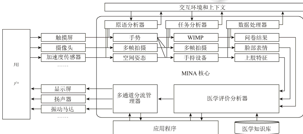
Fig.2 MINA: Multimodal human-computer interaction model for nerve assessment in mobile environment
