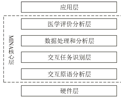
Fig.1 Layered structure of interactive system for nerve function assessment in mobile environment
