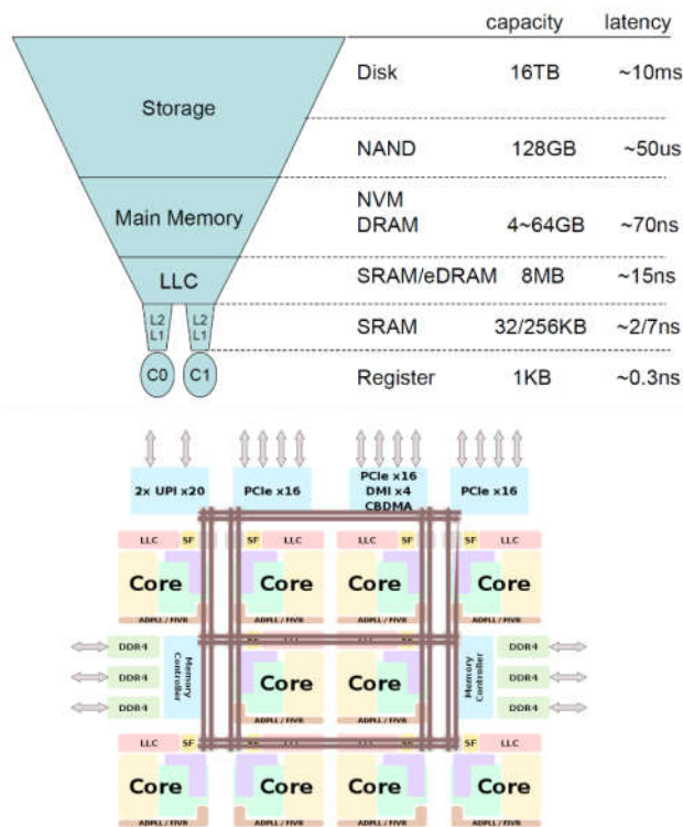
Fig.3 Classical Multi-cores Memory Architecture and recent Intel CPU Microarchitectre
