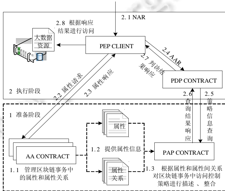
Fig.3 BBAC-BD framework
