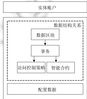
Fig.5 Entity relationship in the block
