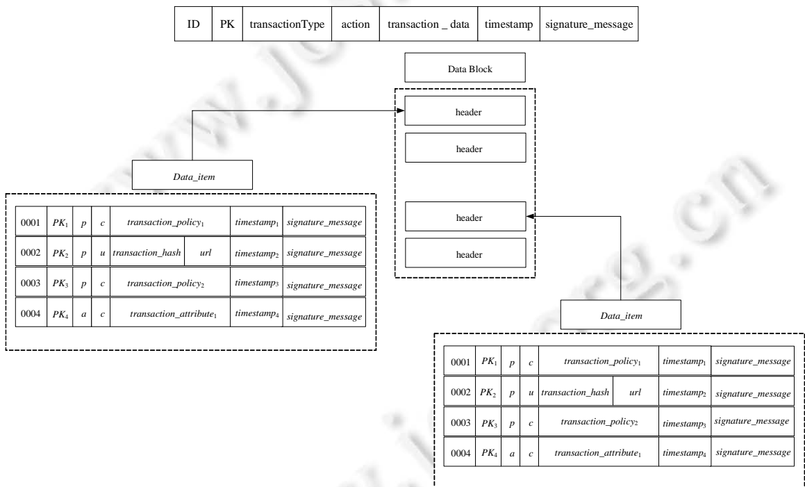
Fig.6 Transaction management level relationship
