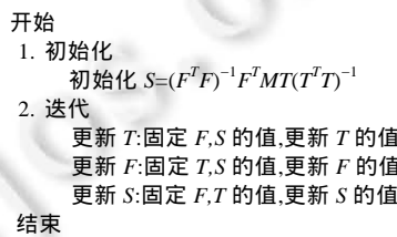
Fig.5 Matrix factorization algorithm
