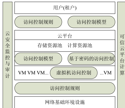
Fig.3 Access control framework in cloud computing environment
