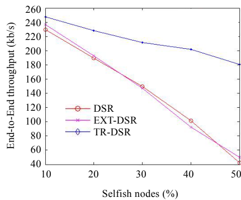
Fig.9 End-to-End throughput vs. selfish nodes ratio
