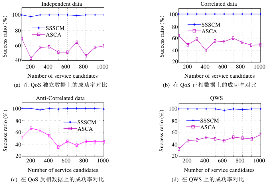
Fig.5 Comparisons on success ratio with SSSCM and ASCA
