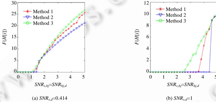
Fig.11 Cooperative gain
