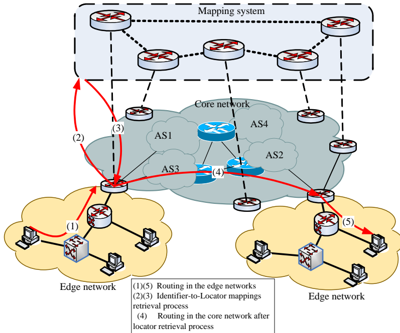
Fig.1 The sketch map of identifier-based routing
