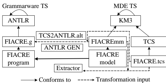
Fig.8 FIACRE model-to-text bridge
