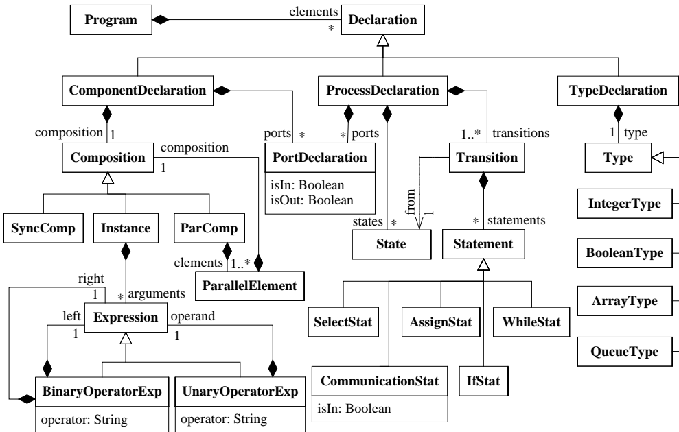
Fig.3 Core metamodel of FIACRE
