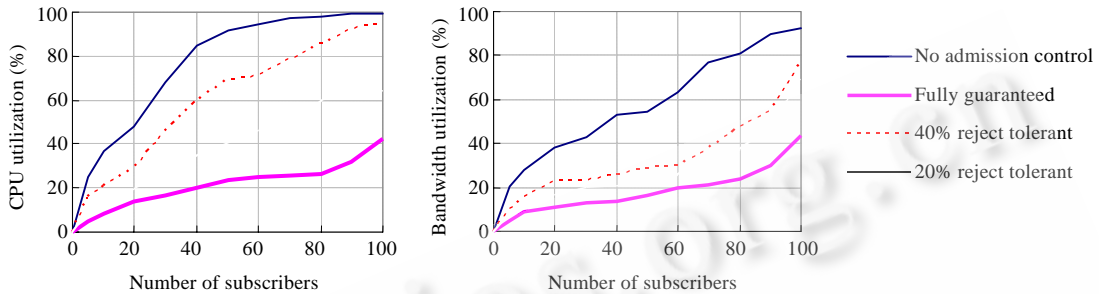
Fig.10 CPU and bandwidth utilization of different strategies
