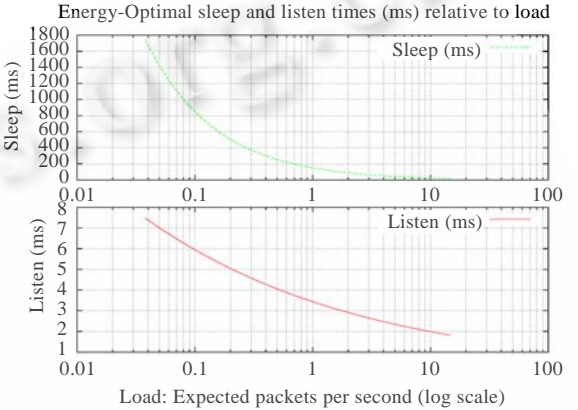
Fig.3 Energy-Optimal sleep and listen times
