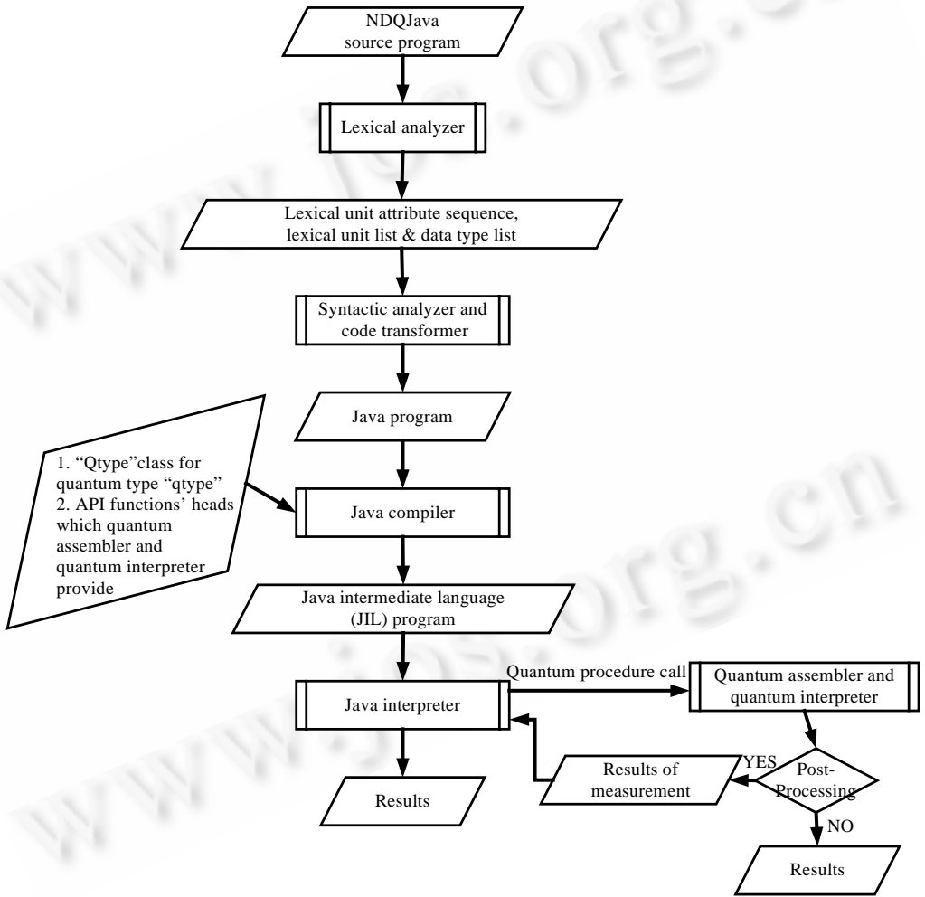
Fig.1 Flow diagram of the NDQJava processing system
