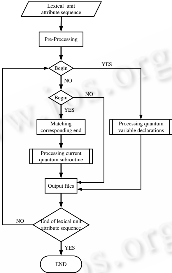
Fig.2 Flow diagram of syntactic analyzer of NDQJava processing system
