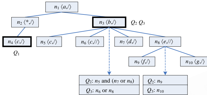
Fig.4 Prefix shared compact query tree 图 4 共享前缀的紧凑查询树
