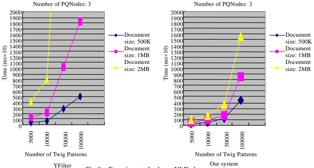
Fig.8 Experiments for large XML documents
