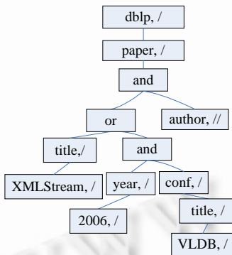
Fig.1 Parse tree of a Twig Pattern 图 1 Twig Pattern 分析树
