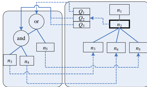
Fig.6 Sharing of common logic expression
