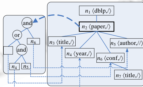
Fig.2 Compact parse tree of a Twig Pattern 图 2 Twig Pattern 紧凑分析树
