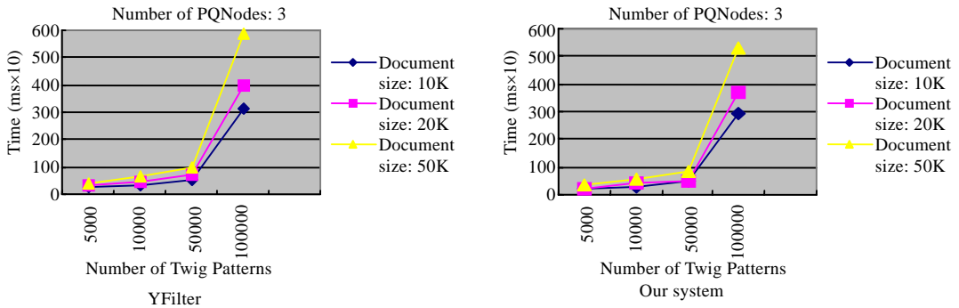
Fig.7 Experiments for small XML documents
