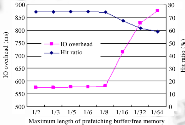
Fig.4 The effect of maximum prefetching buffer length for prefetching algorithm of RAM Grid
