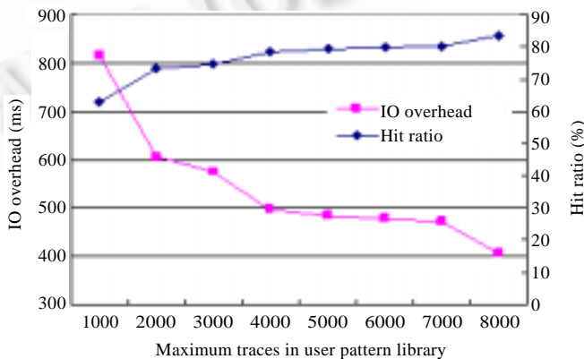
Fig.5 The effect of maximum traces in user pattern library for prefetching algorithm of RAM Grid
