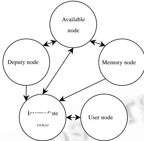
Fig.1 Nodes and their transitions in RAM grid
