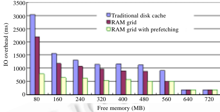
Fig.3 The relationship of the caching effect of RAM grid and local free memory
