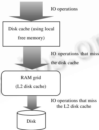
Fig.2 The effect of RAM grid in IO intensive applications
