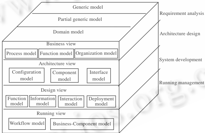
Fig.2 Integrated reference model for adaptive software architecture
