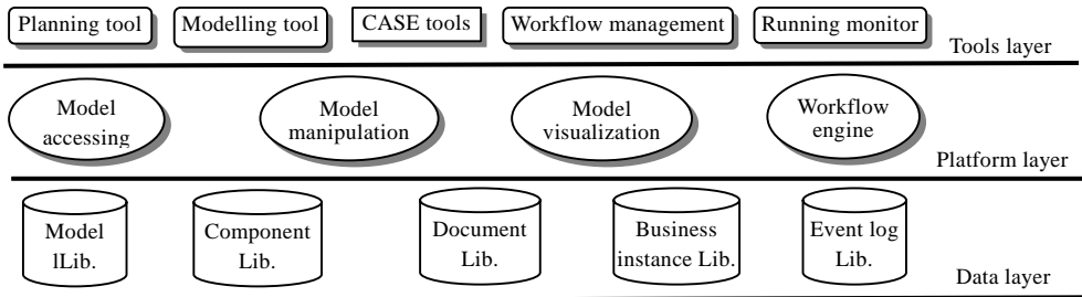
Fig.4 Support tool set for adaptive software architecture
