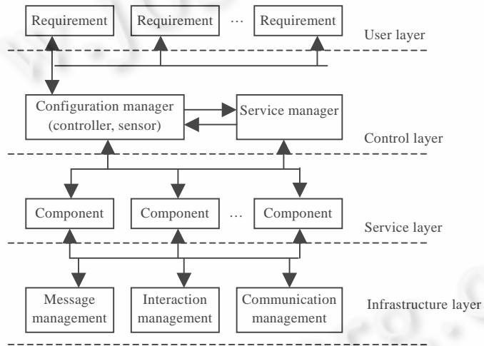
Fig.1 Generic framework for adaptive software architecture
