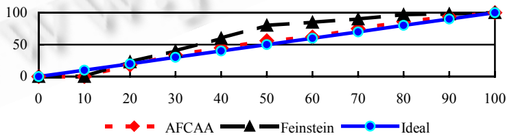
Fig.5 The contrast chart of filter performance in the character of field static attack 图 5 字段固定特征的攻击下包过滤性能对比图
