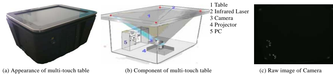
Fig.1 Multi-Touch table
