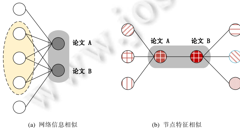
Fig.1 Two similarity in graph
