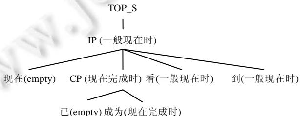
Fig.2 Tagged tense tree
