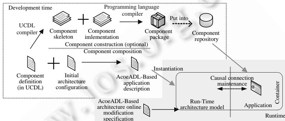
Fig.3 ACOE component construction and composition 图 3 ACOE 构件的构造和组装
