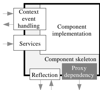
Fig.2 ACOE component skeleton 图 2 ACOE 构件框架
