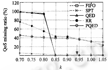
Fig.7 Variation of system capability
