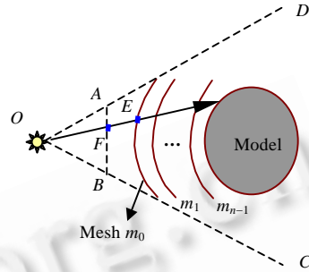
Fig.4 Generating multi-layer shadow maps by rendering scene from the light source of eye
