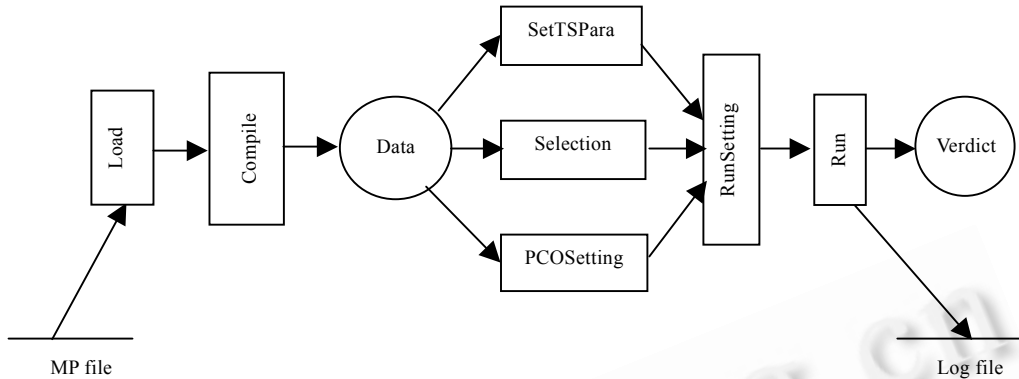
Fig.3 A simplified process of TTCN executor 图3 TTCN 执行器的简化流程
