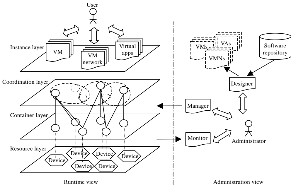
Fig.5 CIVIC system views
