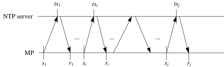
Fig.1 The CPU frequency estimation process
