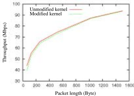
Fig.7 The throughputs of system before and after kernel modification
