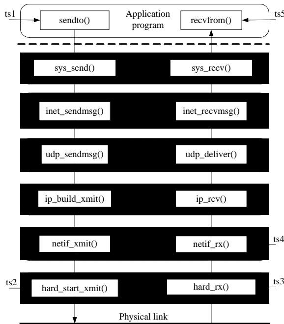
Fig.3 The UDP packet treatment process of Linux
