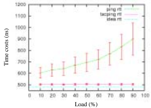
Fig.6 The relation between CPU load and measured RTT
