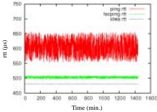
Fig.5 The time series of round trip delay (packet length: 1 500 Byte)
