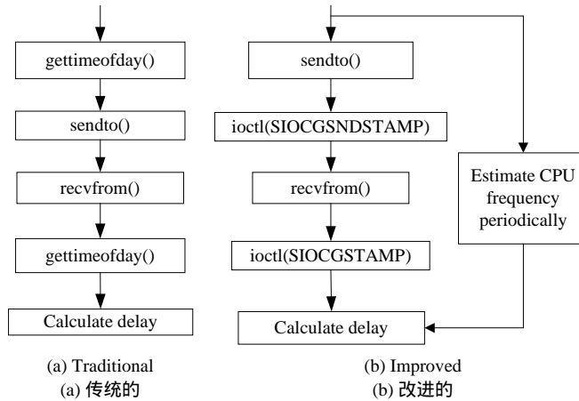
Fig.4 Comparison of delay measurement process
